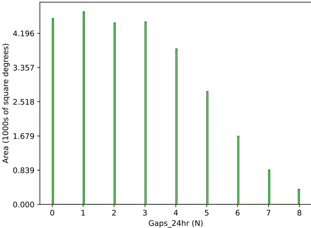
roman_v3.3_10yrs g band: Gaps_24hr
