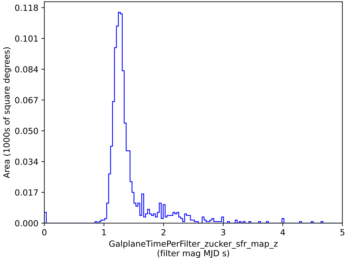
roman_v3.3_10yrs : GalplaneTimePerFilter_zucker_sfr_map_z
