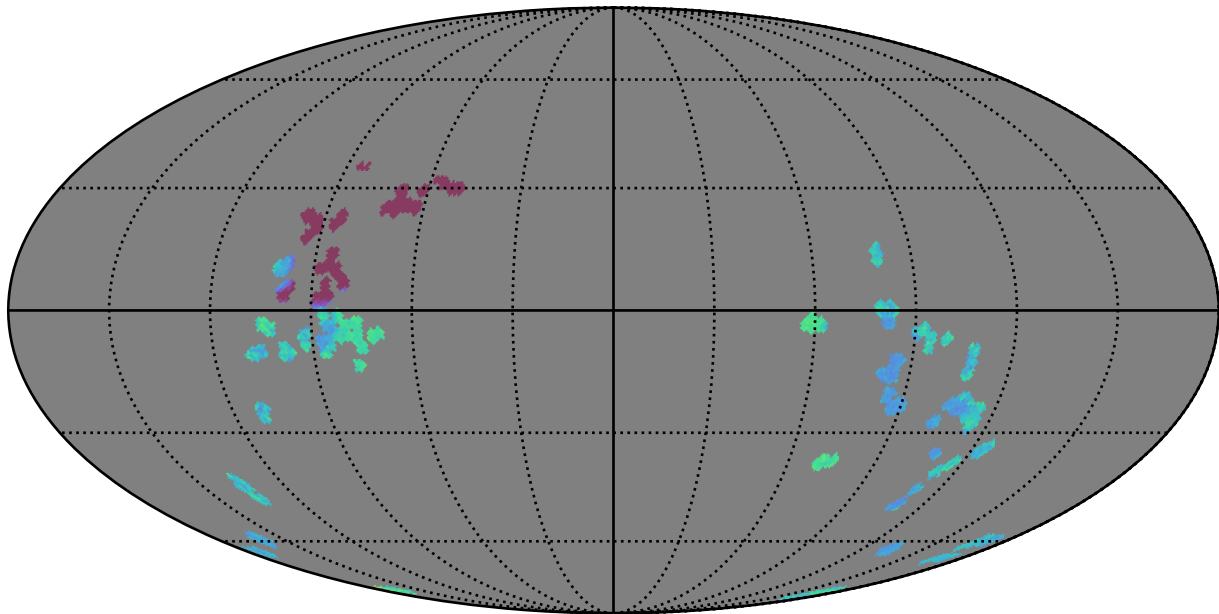
roman_v3.3_10yrs : GalplaneTimePerFilter_zucker_sfr_map_y
