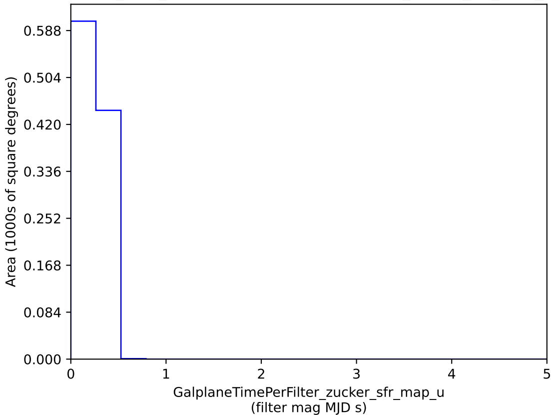
roman_v3.3_10yrs : GalplaneTimePerFilter_zucker_sfr_map_u
