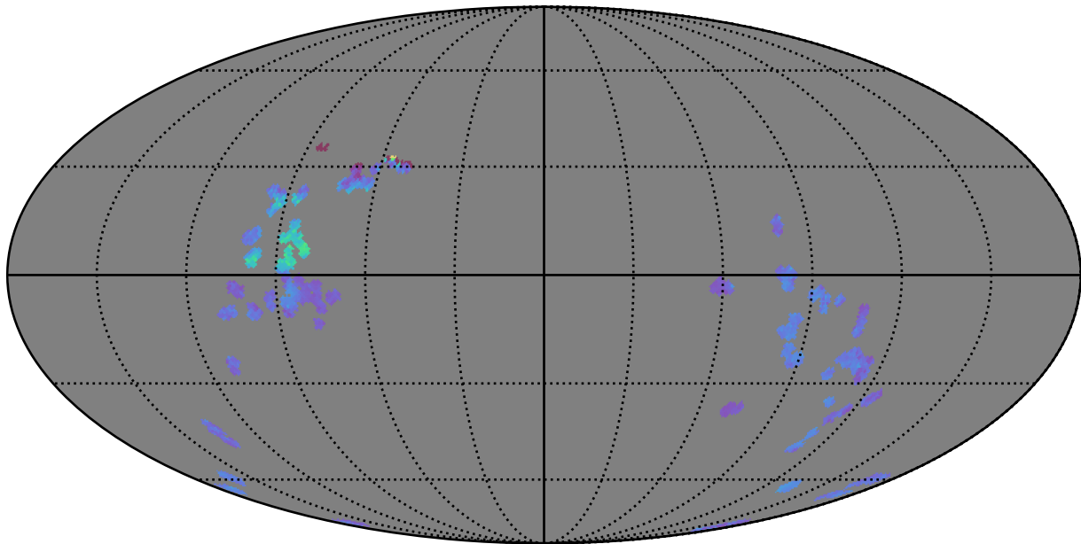
roman_v3.3_10yrs : GalplaneTimePerFilter_zucker_sfr_map_g
