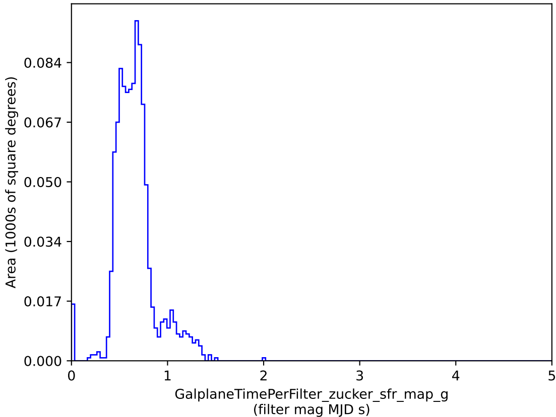
roman_v3.3_10yrs : GalplaneTimePerFilter_zucker_sfr_map_g
