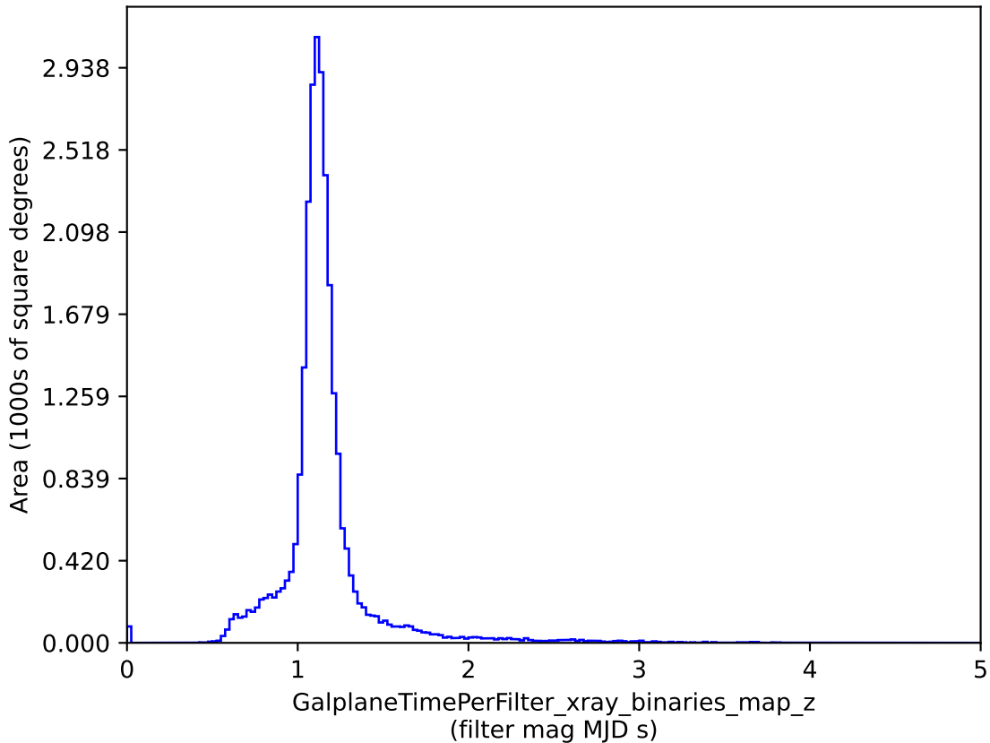
roman_v3.3_10yrs : GalplaneTimePerFilter_xray_binaries_map_z
