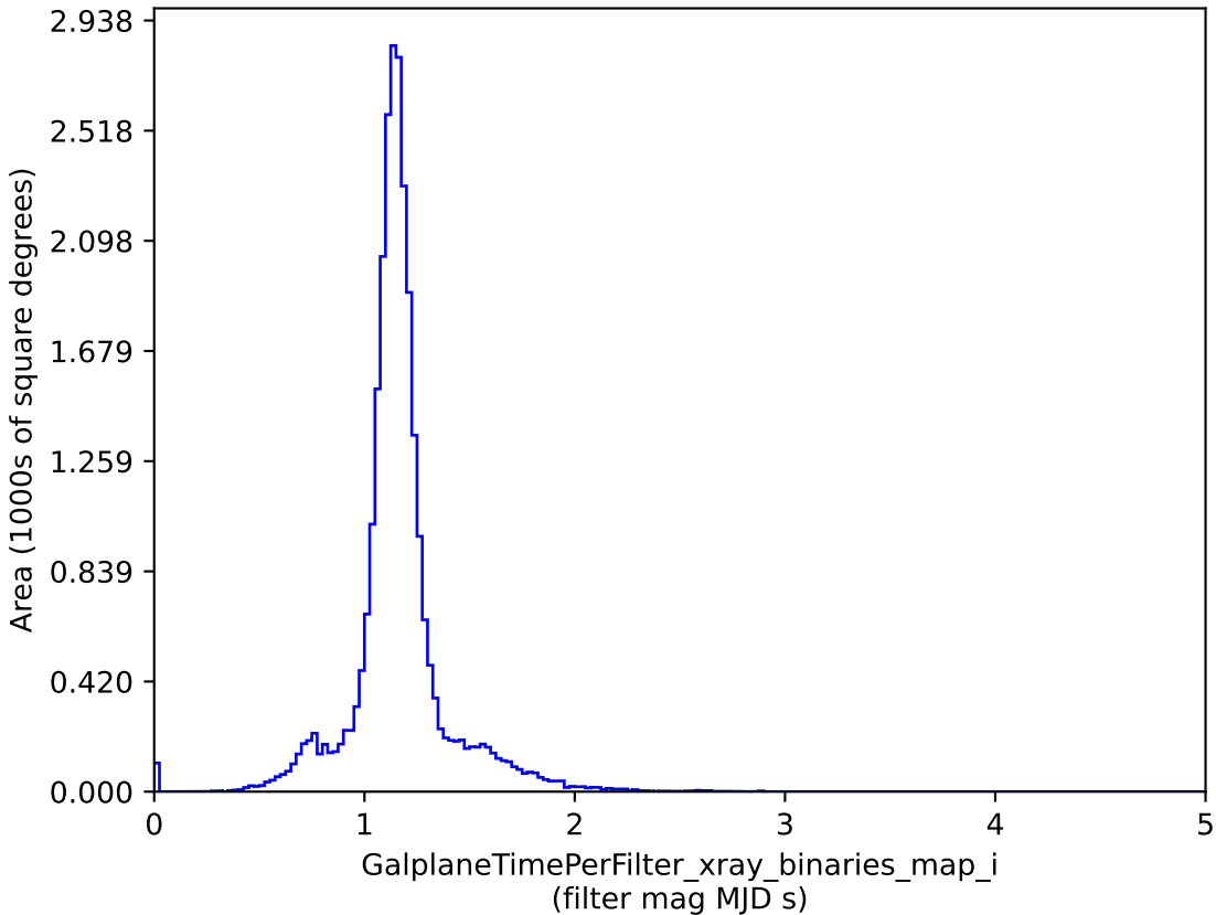
roman_v3.3_10yrs : GalplaneTimePerFilter_xray_binaries_map_i
