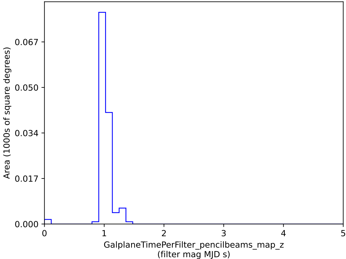
roman_v3.3_10yrs : GalplaneTimePerFilter_pencilbeams_map_z
