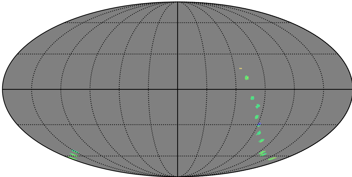
roman_v3.3_10yrs : GalplaneTimePerFilter_pencilbeams_map_y
