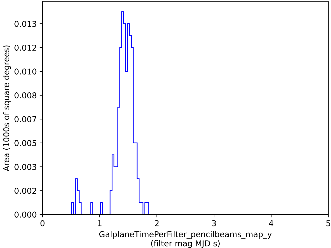
roman_v3.3_10yrs : GalplaneTimePerFilter_pencilbeams_map_y
