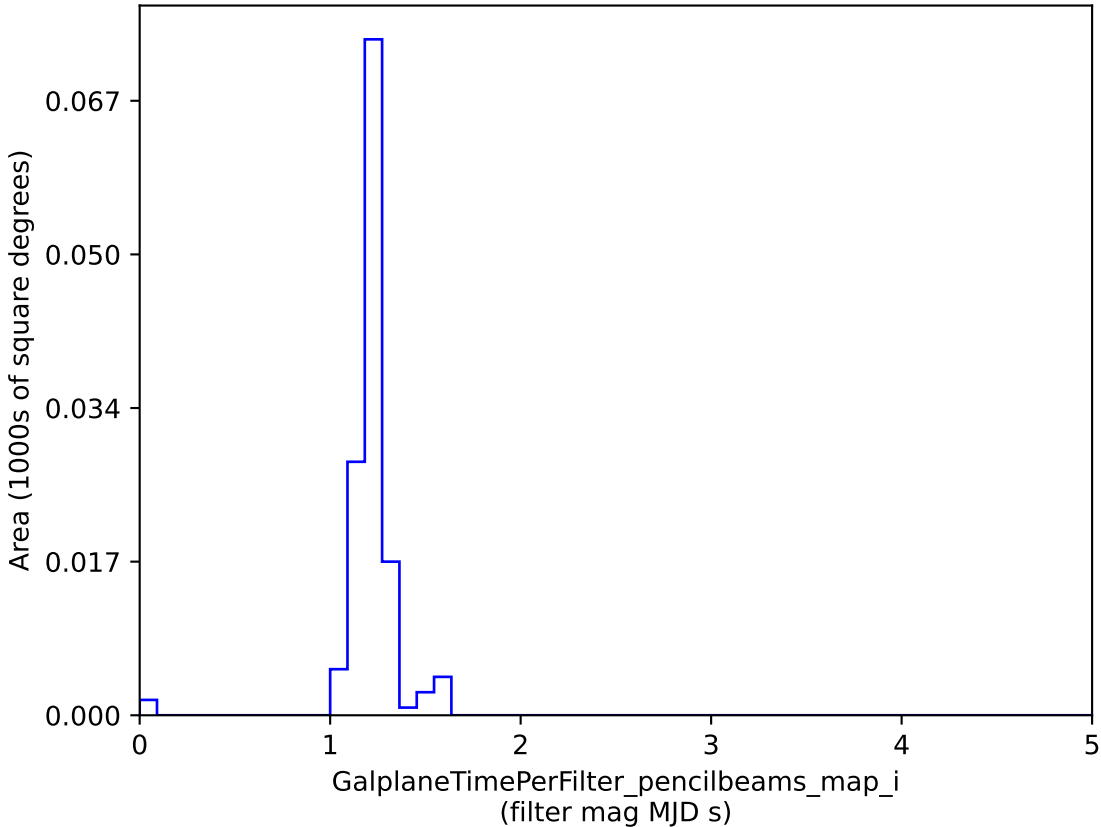
roman_v3.3_10yrs : GalplaneTimePerFilter_pencilbeams_map_i
