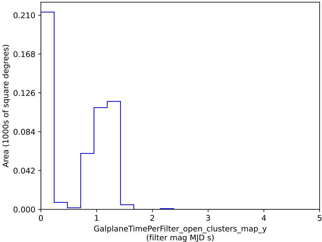
roman_v3.3_10yrs : GalplaneTimePerFilter_open_clusters_map_y
