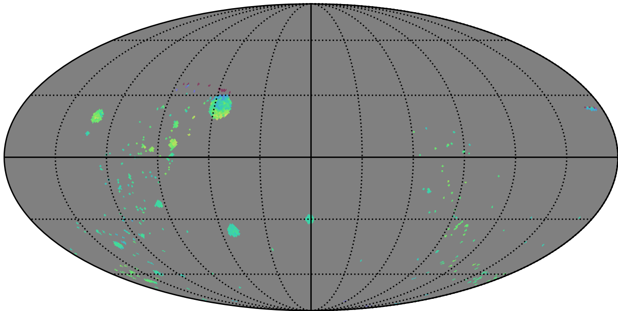
roman_v3.3_10yrs : GalplaneTimePerFilter_open_clusters_map_r
