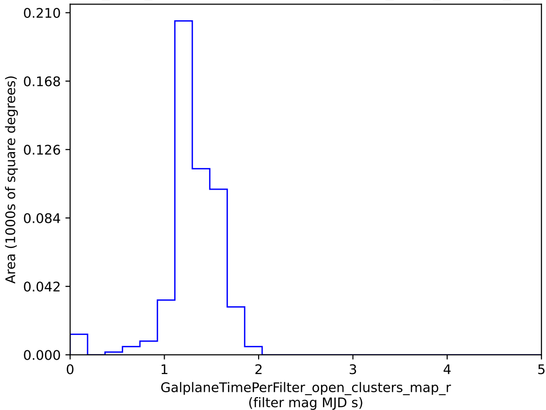
roman_v3.3_10yrs : GalplaneTimePerFilter_open_clusters_map_r
