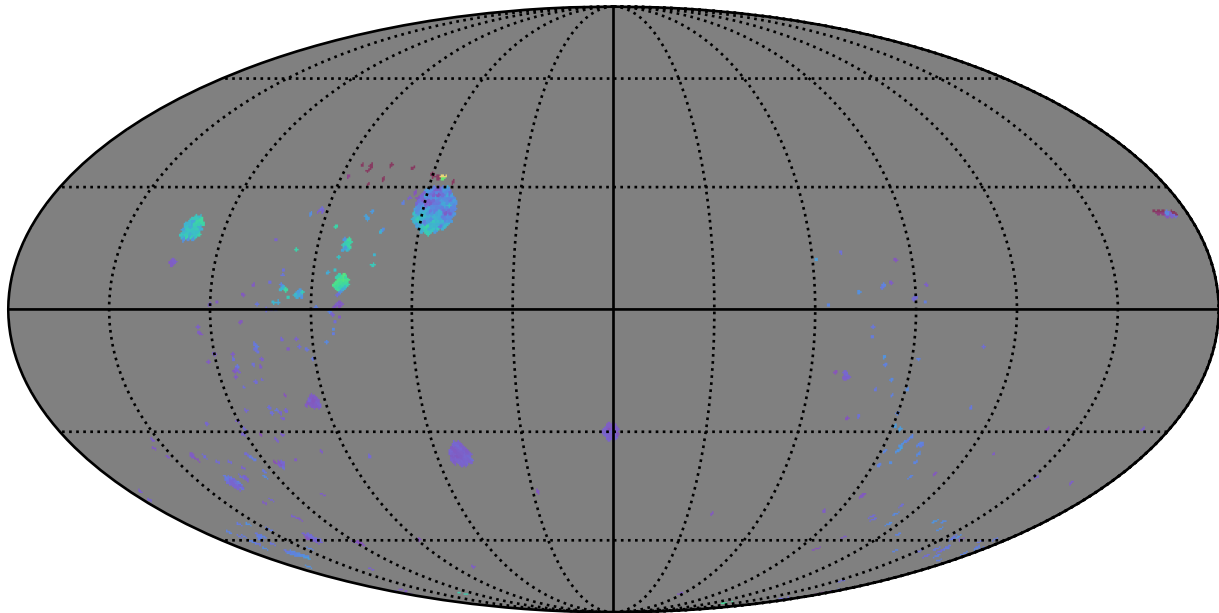
roman_v3.3_10yrs : GalplaneTimePerFilter_open_clusters_map_g
