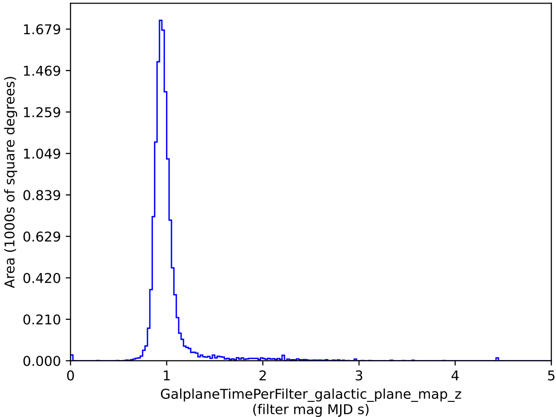
roman_v3.3_10yrs : GalplaneTimePerFilter_galactic_plane_map_z
