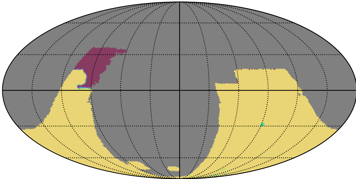
roman_v3.3_10yrs : GalplaneTimePerFilter_galactic_plane_map_y
