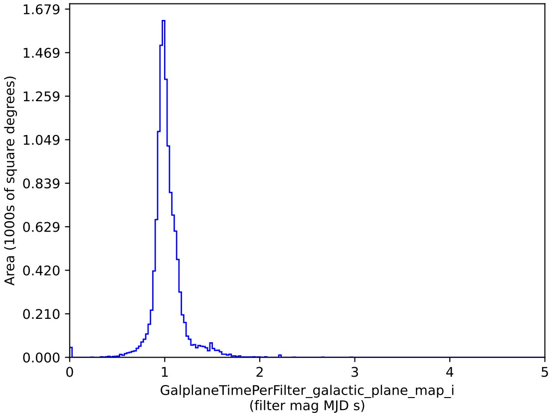
roman_v3.3_10yrs : GalplaneTimePerFilter_galactic_plane_map_i
