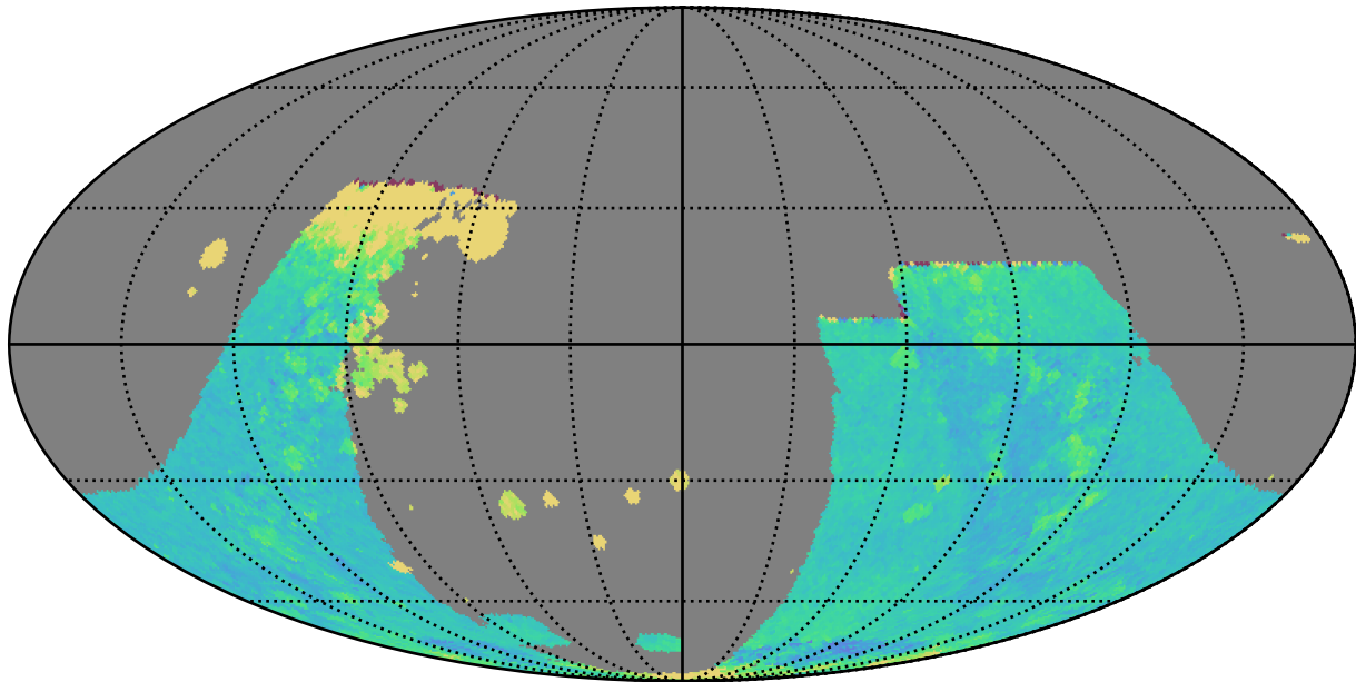
roman_v3.3_10yrs : GalplaneTimePerFilter_combined_map_z
