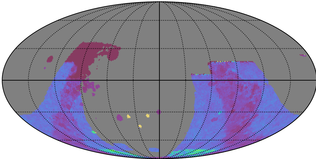
roman_v3.3_10yrs : GalplaneTimePerFilter_combined_map_u
