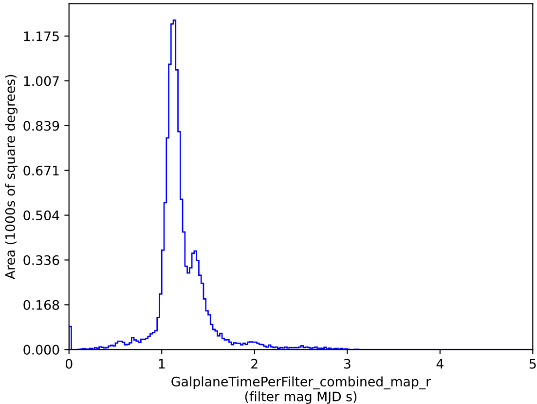
roman_v3.3_10yrs : GalplaneTimePerFilter_combined_map_r
