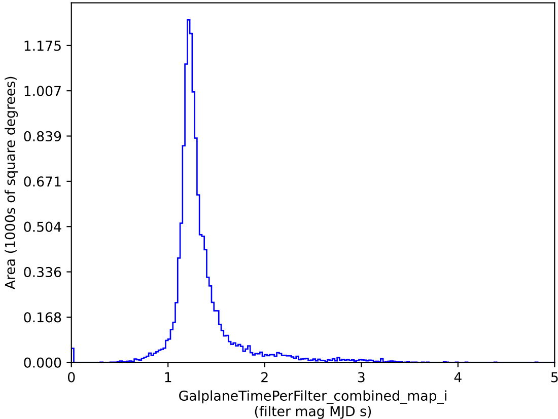
roman_v3.3_10yrs : GalplaneTimePerFilter_combined_map_i
