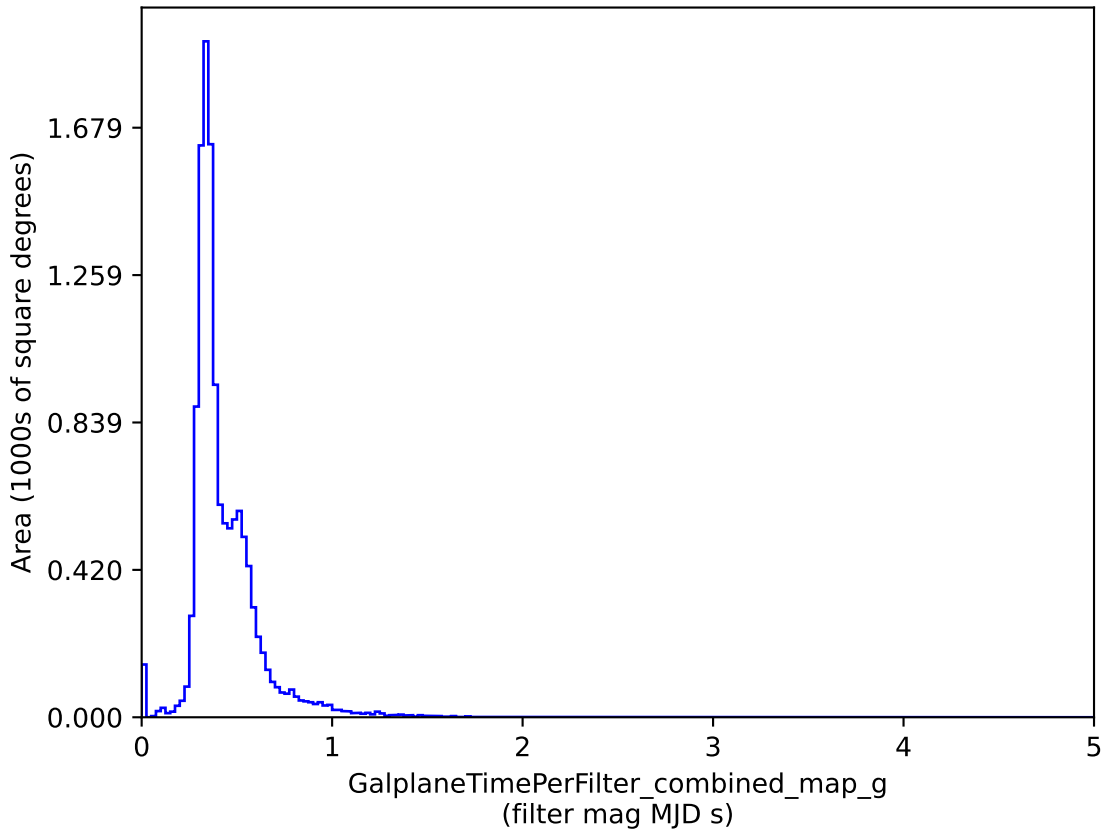
roman_v3.3_10yrs : GalplaneTimePerFilter_combined_map_g
