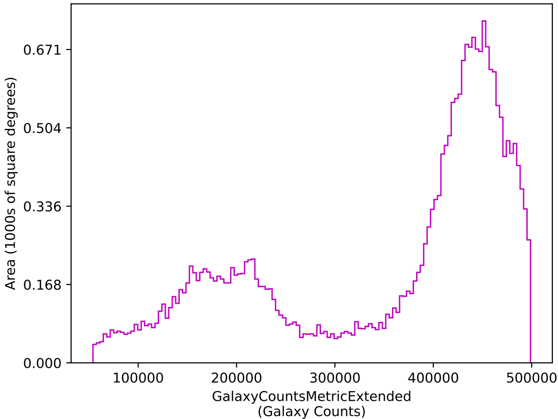
roman_v3.3_10yrs z: GalaxyCountsMetricExtended
