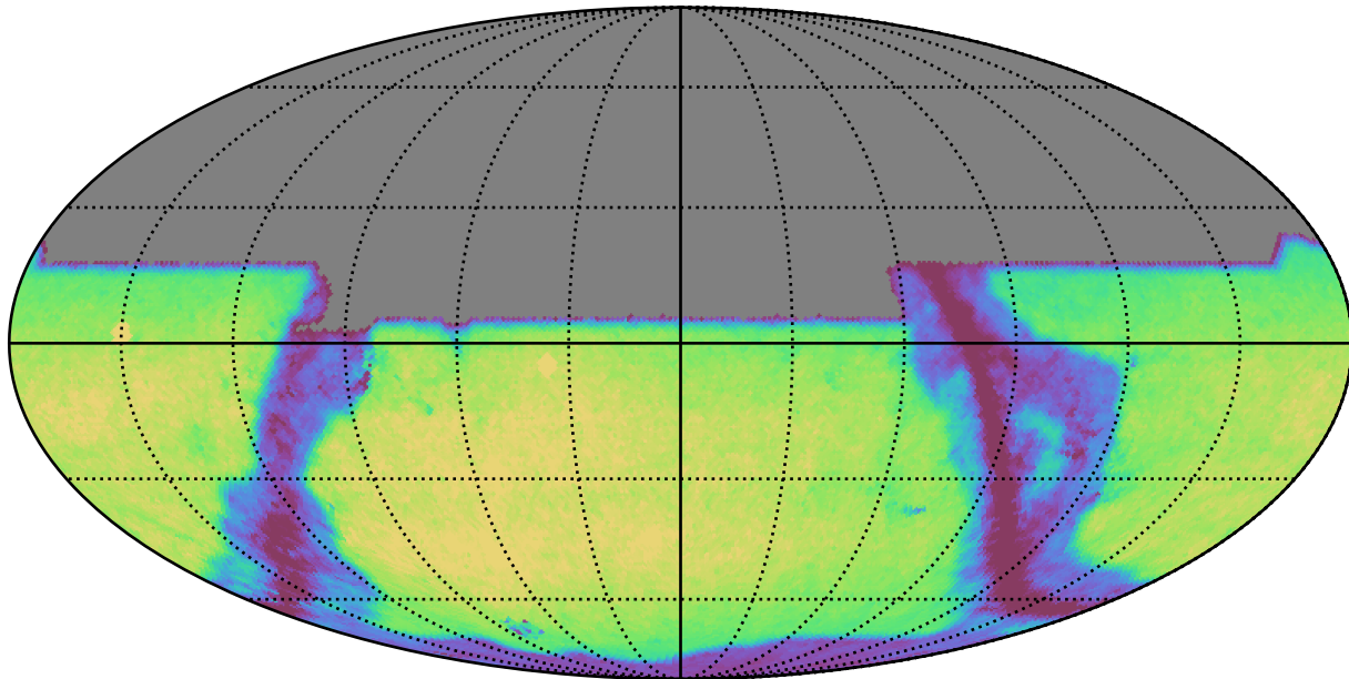
roman_v3.3_10yrs y: GalaxyCountsMetricExtended
