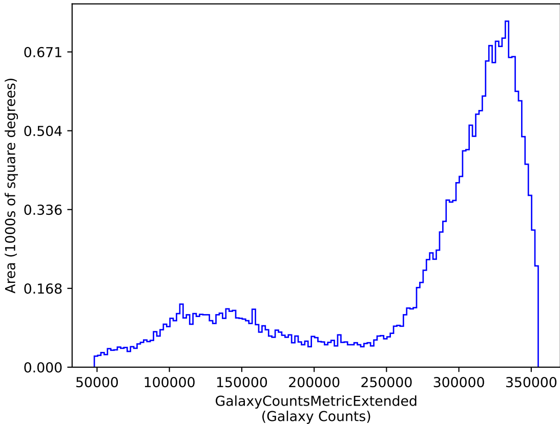
roman_v3.3_10yrs y: GalaxyCountsMetricExtended
