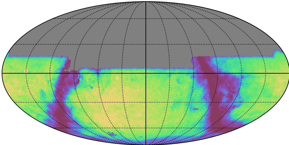
roman_v3.3_10yrs u: GalaxyCountsMetricExtended
