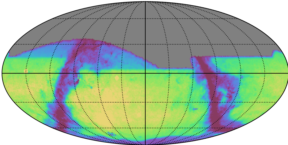
roman_v3.3_10yrs r: GalaxyCountsMetricExtended
