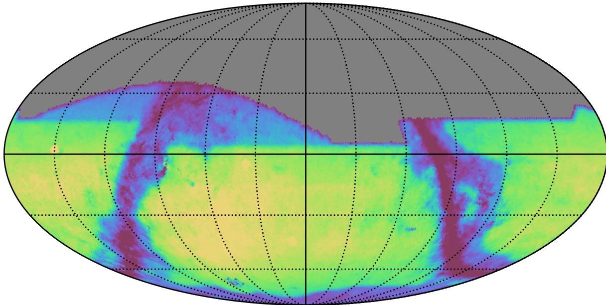
roman_v3.3_10yrs i: GalaxyCountsMetricExtended
