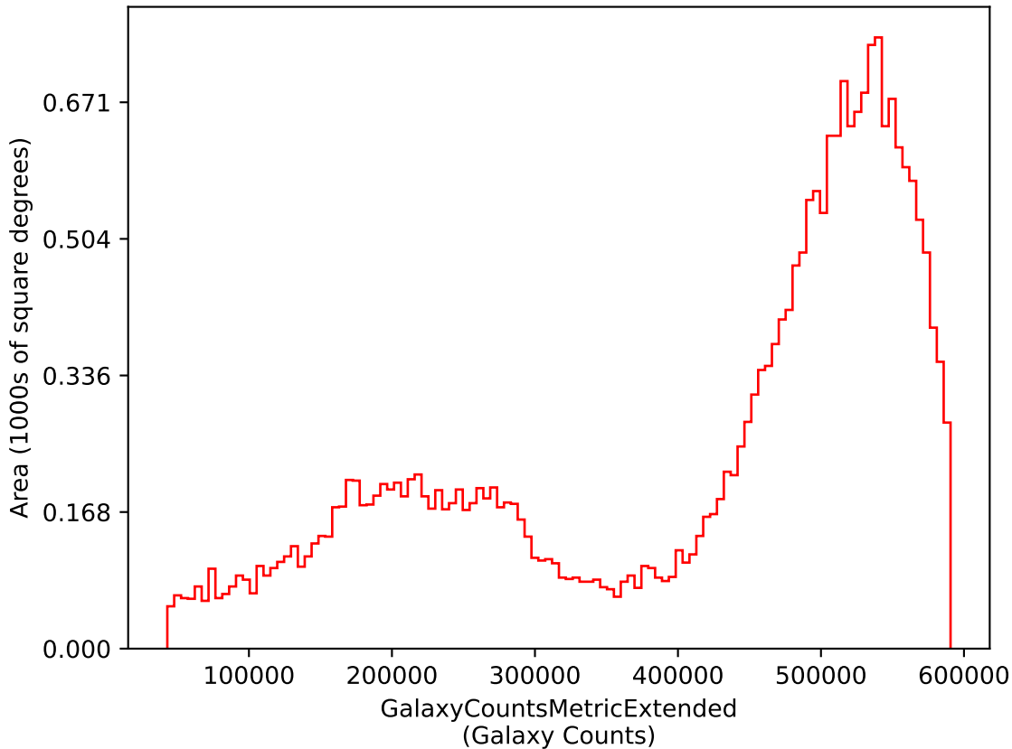
roman_v3.3_10yrs i: GalaxyCountsMetricExtended
