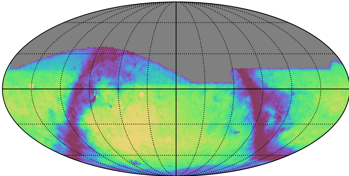
roman_v3.3_10yrs g: GalaxyCountsMetricExtended
