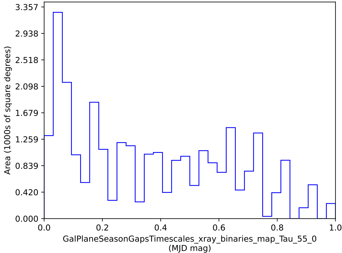
roman_v3.3_10yrs : GalPlaneSeasonGapsTimescales_xray_binaries_map_Tau_55_0
