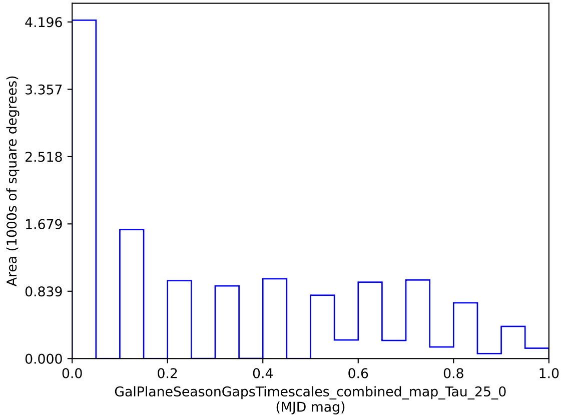
roman_v3.3_10yrs : GalPlaneSeasonGapsTimescales_combined_map_Tau_25_0
