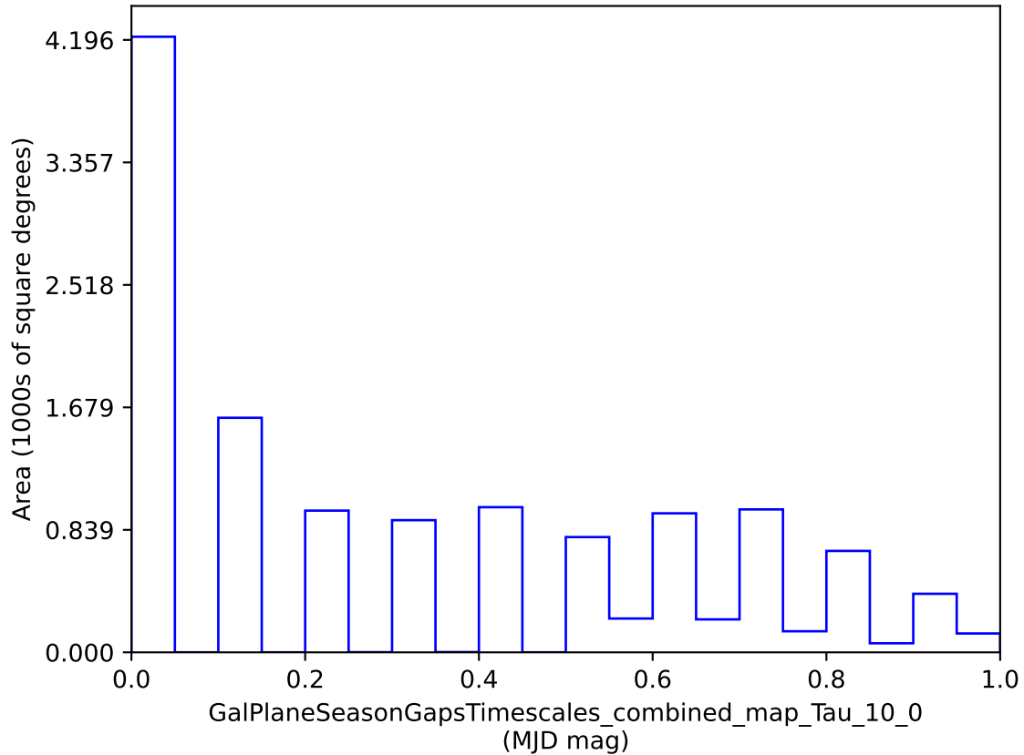
roman_v3.3_10yrs : GalPlaneSeasonGapsTimescales_combined_map_Tau_10_0
