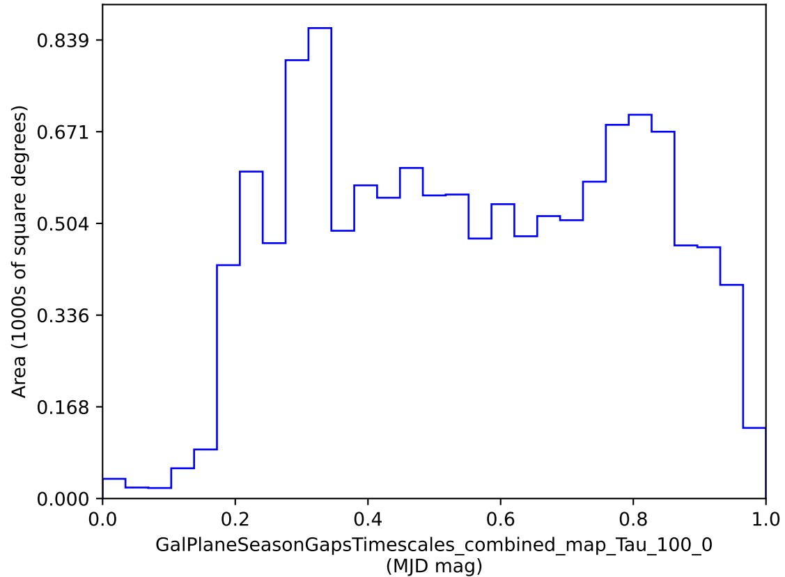
roman_v3.3_10yrs : GalPlaneSeasonGapsTimescales_combined_map_Tau_100_0
