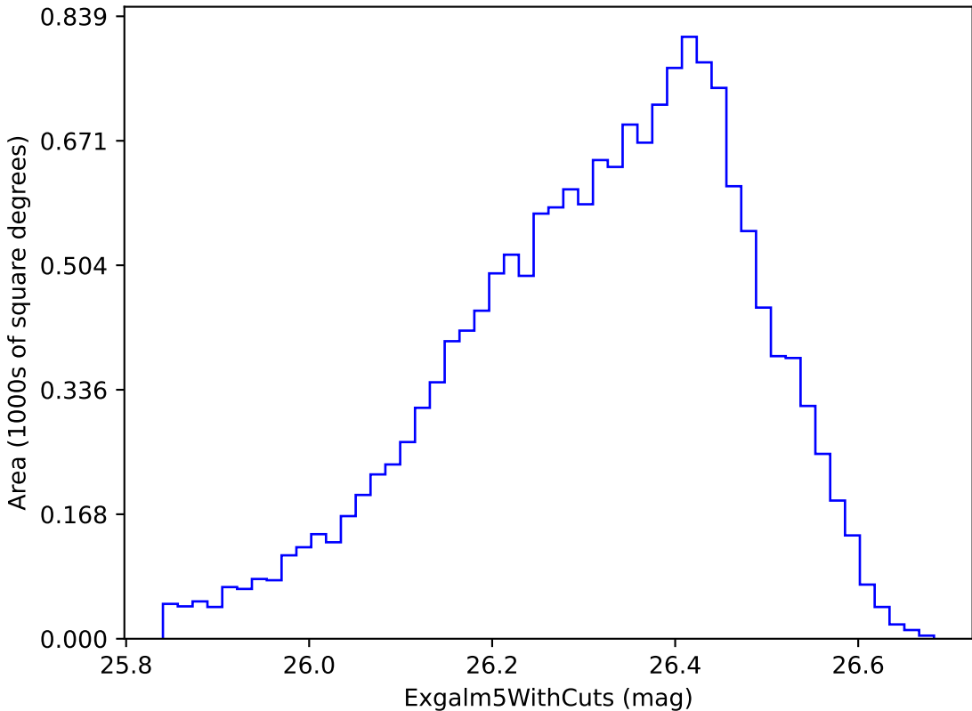
roman_v3.3_10yrs i band non-DD year 9: ExgalM5WithCuts
