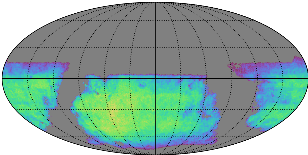
roman_v3.3_10yrs i band non-DD year 8: Exgalml5WithCuts
