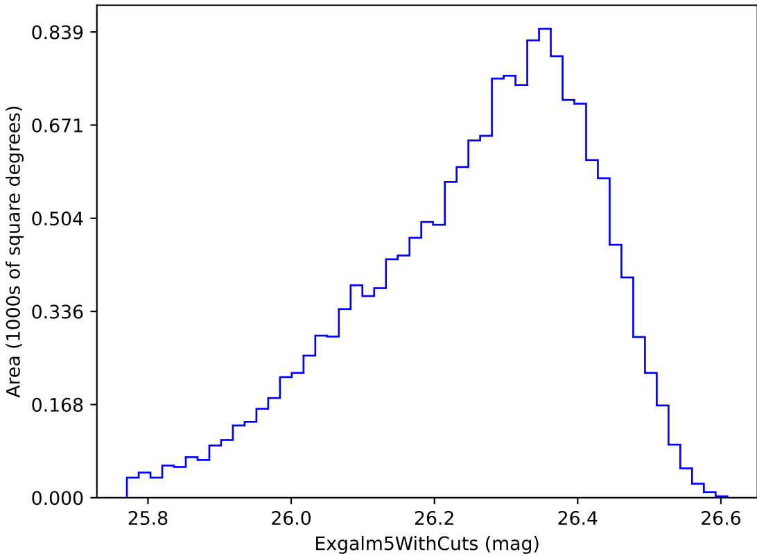
roman_v3.3_10yrs i band non-DD year 8: ExgalM5WithCuts
