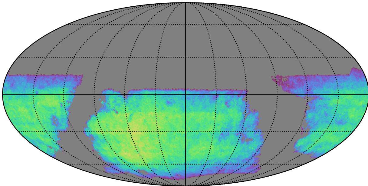
roman_v3.3_10yrs i band non-DD year 6: ExgalM5WithCuts
