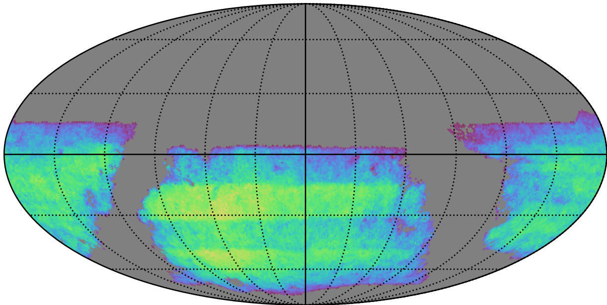
roman_v3.3_10yrs i band non-DD year 5: Exgal5WithCuts
