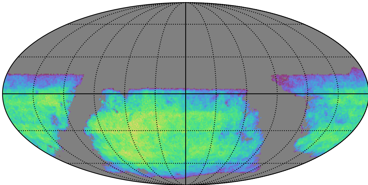
roman_v3.3_10yrs i band non-DD year 4: ExgalM5WithCuts
