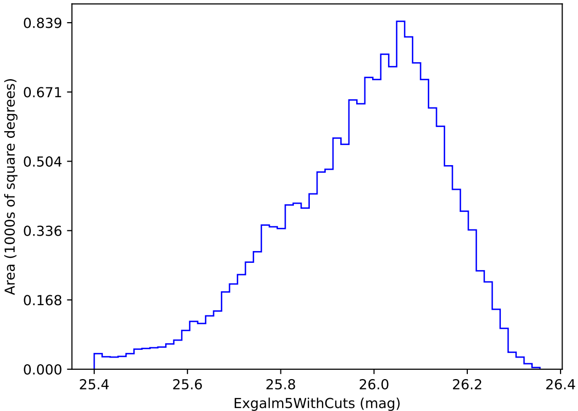
roman_v3.3_10yrs i band non-DD year 4: ExgalM5WithCuts
