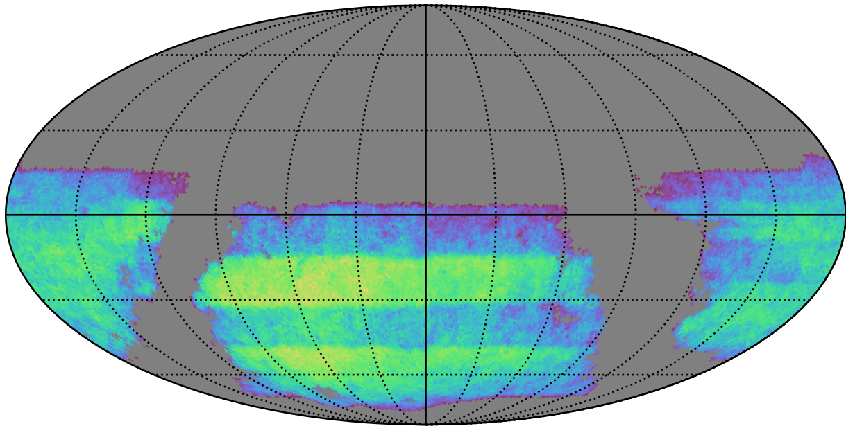
roman_v3.3_10yrs i band non-DD year 3: ExgalM5WithCuts
