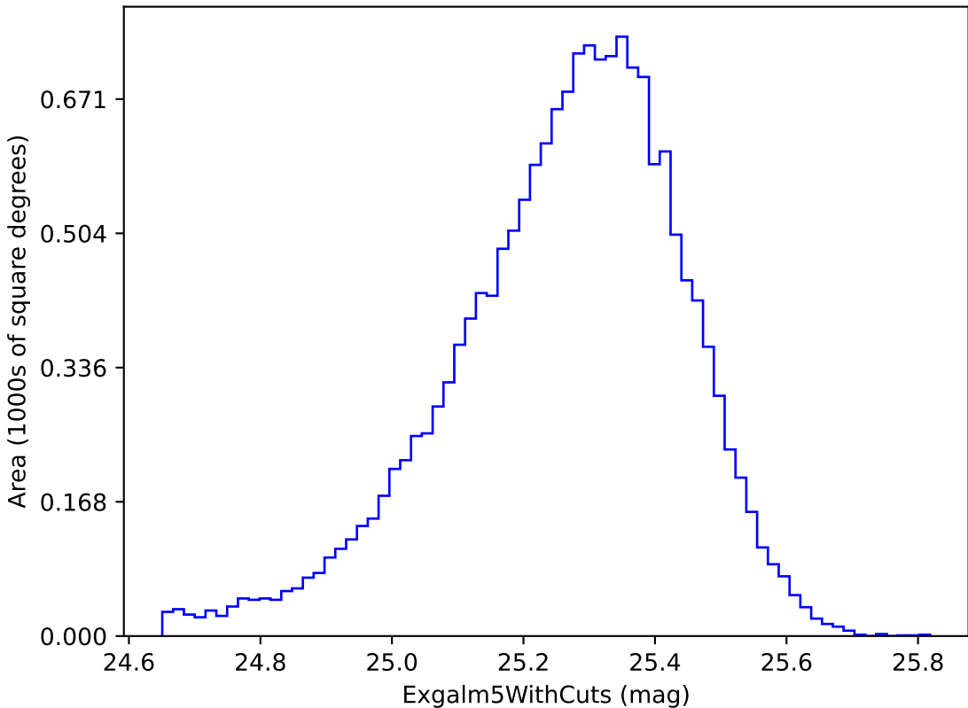
roman_v3.3_10yrs i band non-DD year 1: ExgalM5WithCuts
