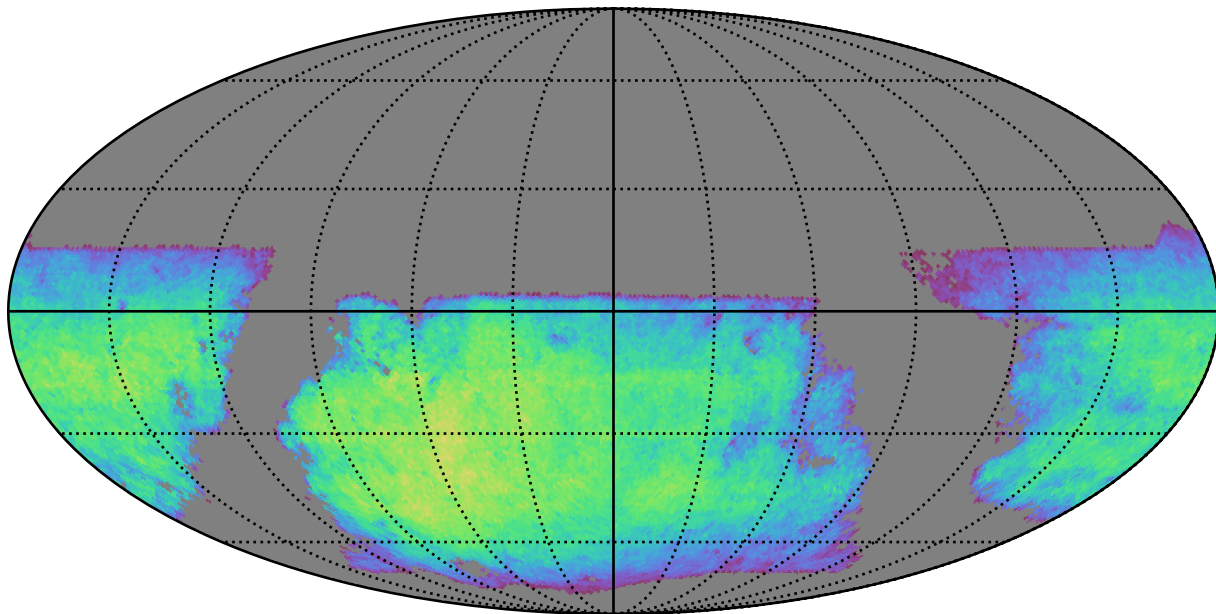
roman_v3.3_10yrs i band non-DD year 10: ExgalM5WithCuts
