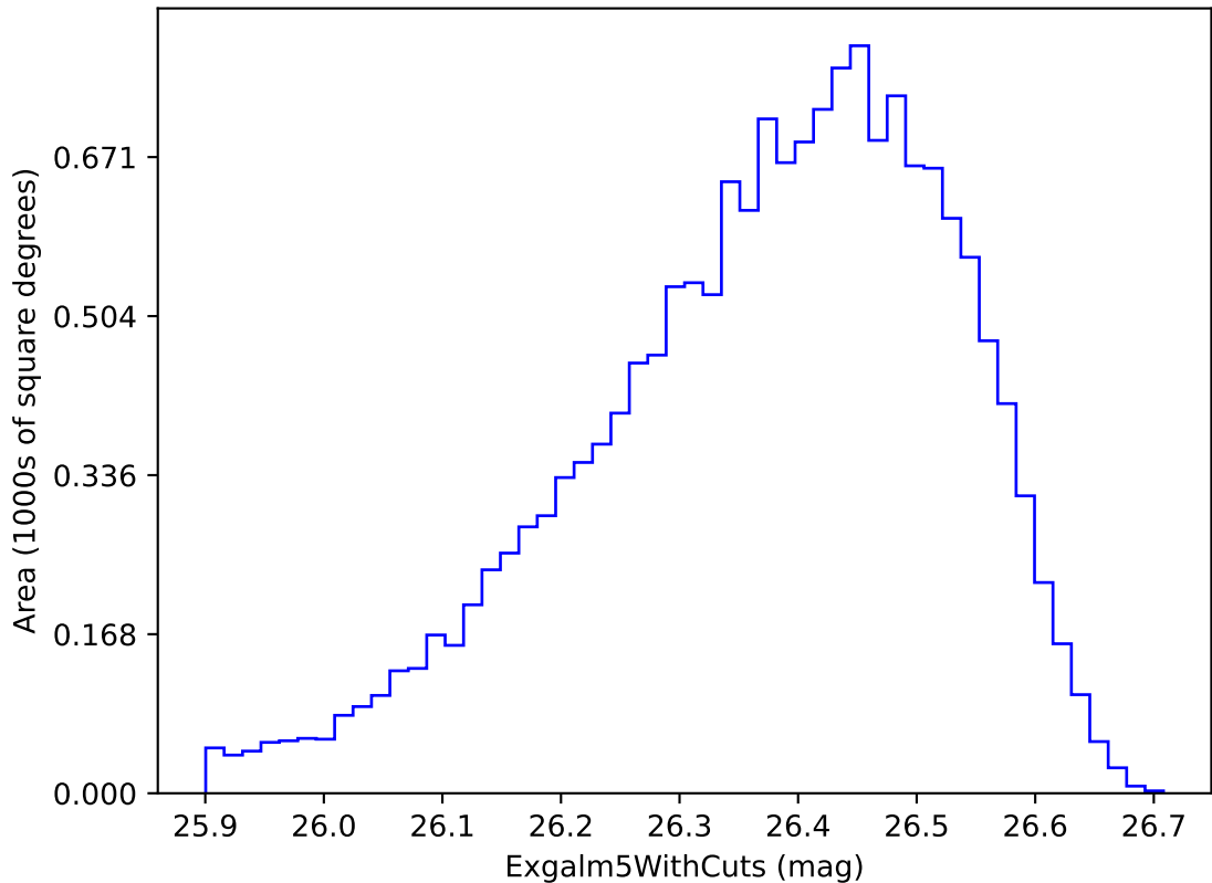
roman_v3.3_10yrs i band non-DD year 10: ExgalM5WithCuts
