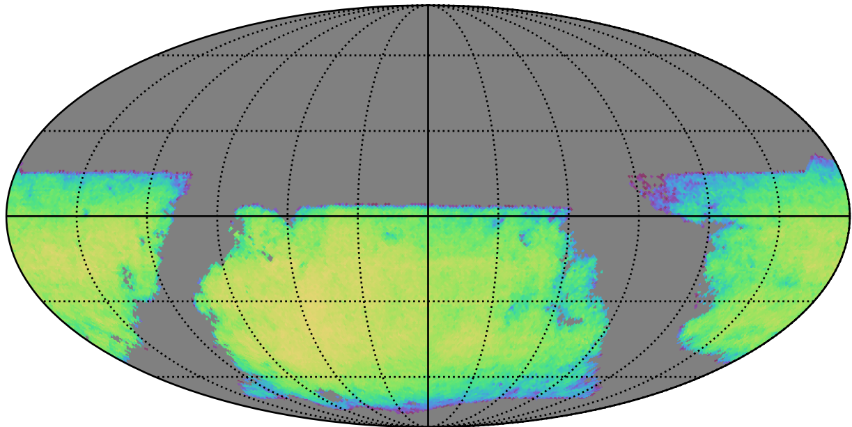
roman_v3.3_10yrs i band galaxies non-DD: DepthLimitedNumGalaxiesMetric
