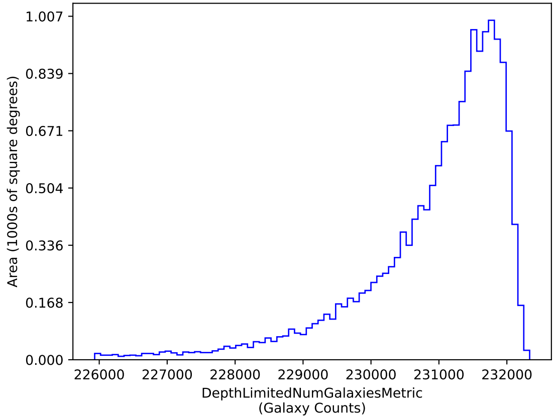
roman_v3.3_10yrs i band galaxies non-DD: DepthLimitedNumGalaxiesMetric
