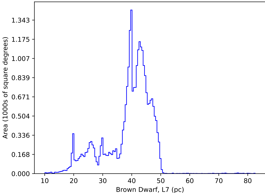
roman_v3.3_10yrs : Brown Dwarf, L7
